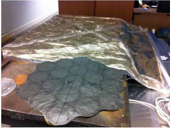
Figure 4: The two inflatable payloads, FRODO in the back and SAM in the front
