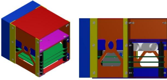
Figure 7: PCBs and batteries within ejectable module
