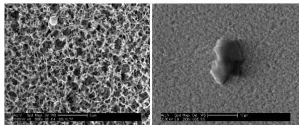
Figure 6. (Left) SEM image of a of 1 \mu\text{m} dia. fluorescent bead on sample collection filter, see top centre-left of image. (Right) SEM image of ~10 \mu\text{m} dia. particle on sample collection filter.
